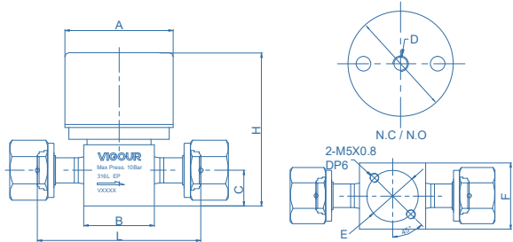
1/2 pneumatic actuator (VFS female)
