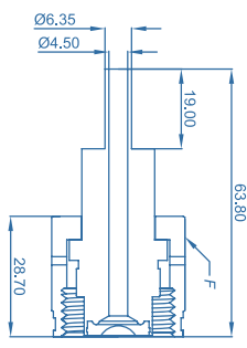
1/4" Tube Weld
