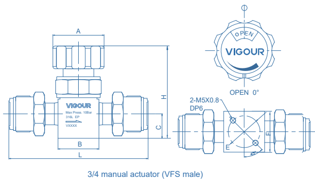
3/4 manual actuator (VFS male)
