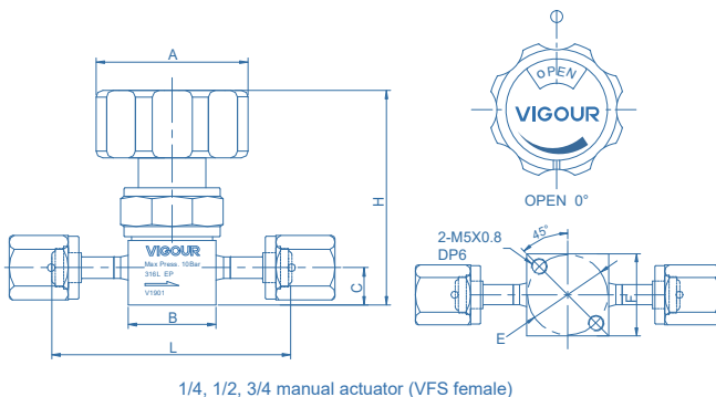
1/4, 1/2, 3/4 manual actuator (VFS female)
