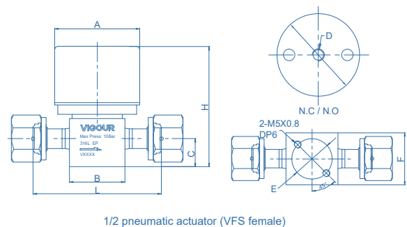
1/2 pneumatic actuator (VFS female)
