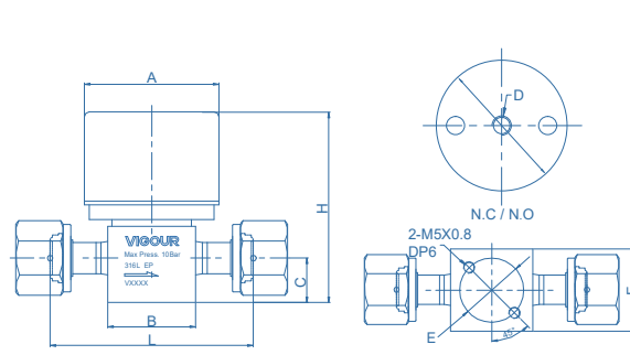
1/2 pneumatic actuator (VFS female)
