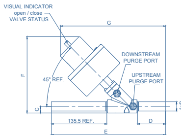
Pneumatic actuator 1"
