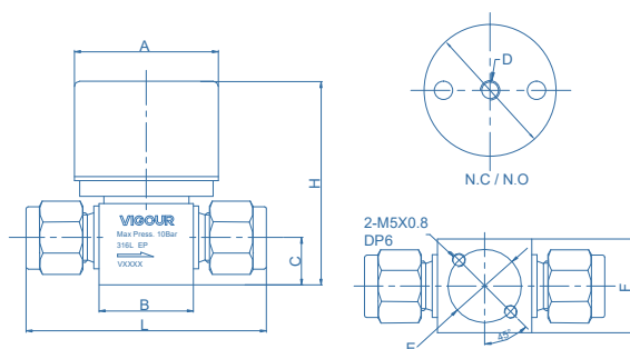
3/8, 1/2 pneumatic actuator
