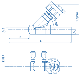
Manual Actuator 3/4~1"
