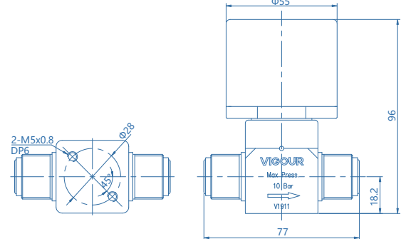
1/2 pneumatic actuator (VFS fitting male)
