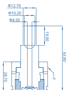
1/2"Weld Tube
